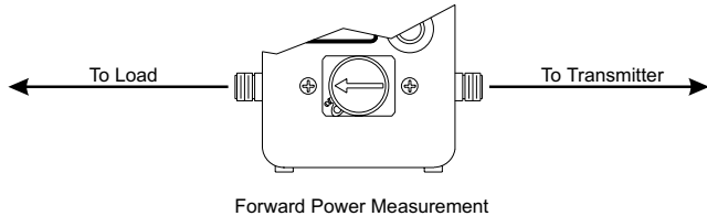
Figure 5 Measurement Direction
